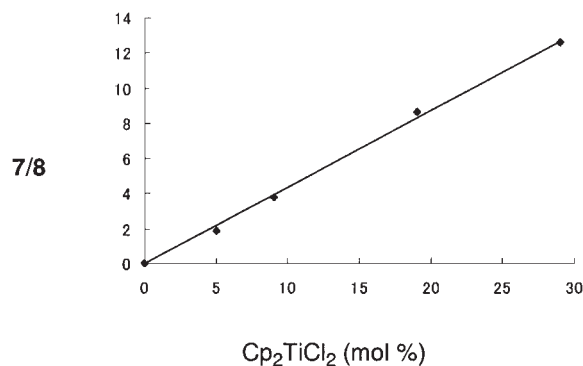
Fig. 1. A plot of 7/8 for the amount of titanocene catalyst. The reactions were run in the presence of 5, 9, 19, and 30 mol% of [\text{Cp}_2\text{TiCl}_2] , 2 mmol of styrene, 1.5 equiv of cyclohexyl bromide, 2.5 equiv of ^n\text{BuMgCl} in 5 mL of \text{Et}_2\text{O} at 0^\circ\text{C} .
