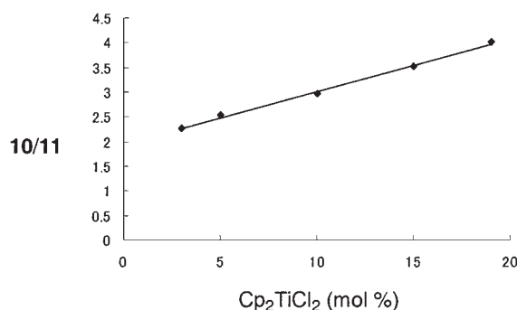
Fig. 2. A plot of 10/11 for the amount of titanocene catalyst. The reactions were run in the presence of 3, 5, 10, 15, and 19 mol% of [\text{Cp}_2\text{TiCl}_2] , 1 equiv of 5-hexenyl bromide, 3 equiv of styrene, 1.3 equiv of n\text{BuMgCl} in 1.3 mL of \text{Et}_2\text{O} at 0 °C for 30 min.
